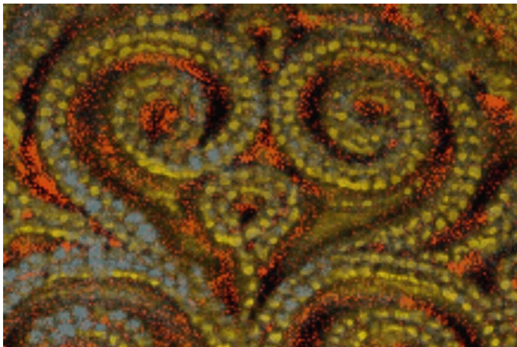
Fig. 14. Detail of filigree on upper foot of Suger Chalice (fig. 1), false color XRF elemental map showing the presence of gold on the surface (yellow), underlying silver where the gold is worn (gray), and iron in the recesses of the design (red).
